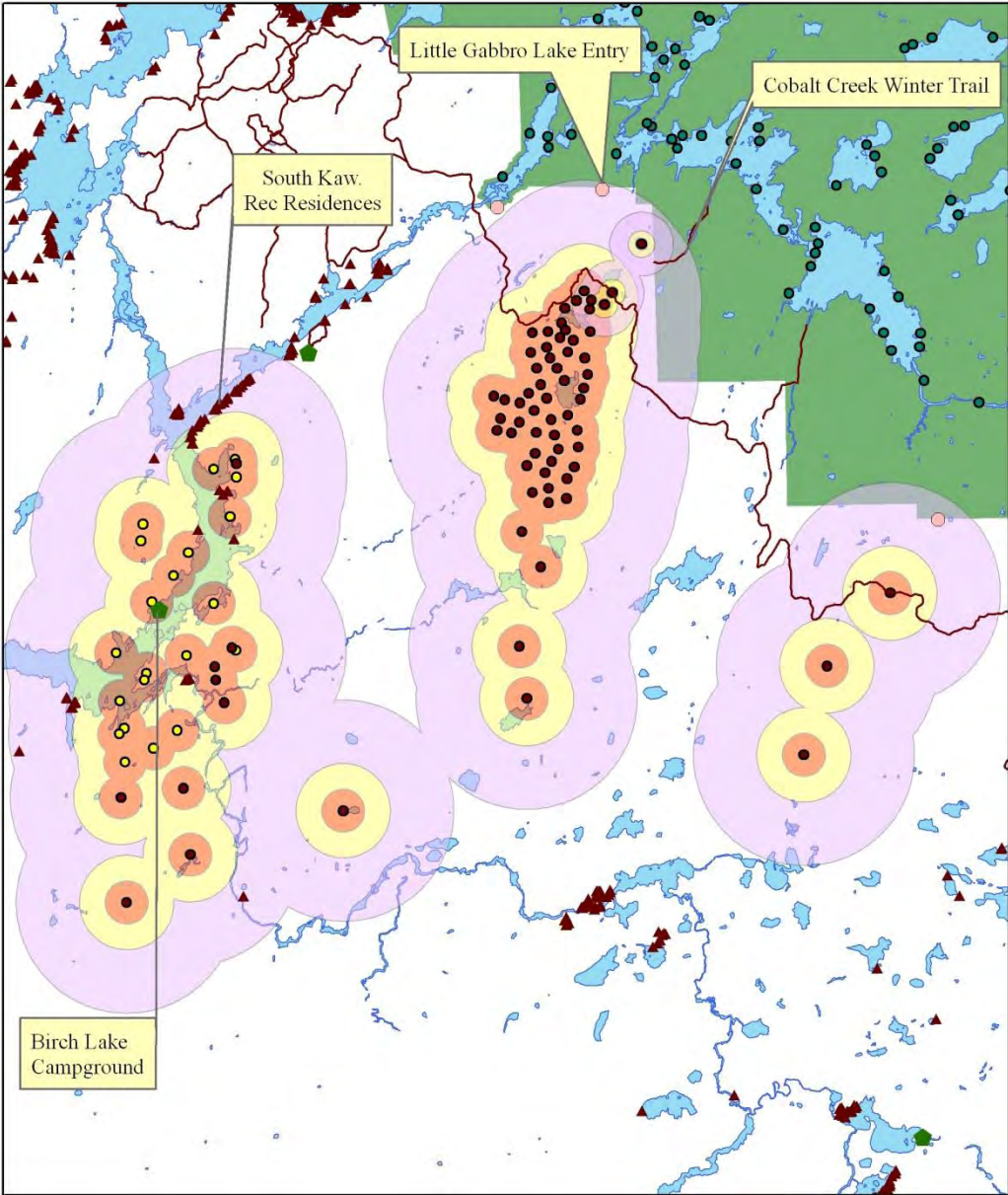
Figure 18 A-weighted sound levels at receptors for Alternative 4
