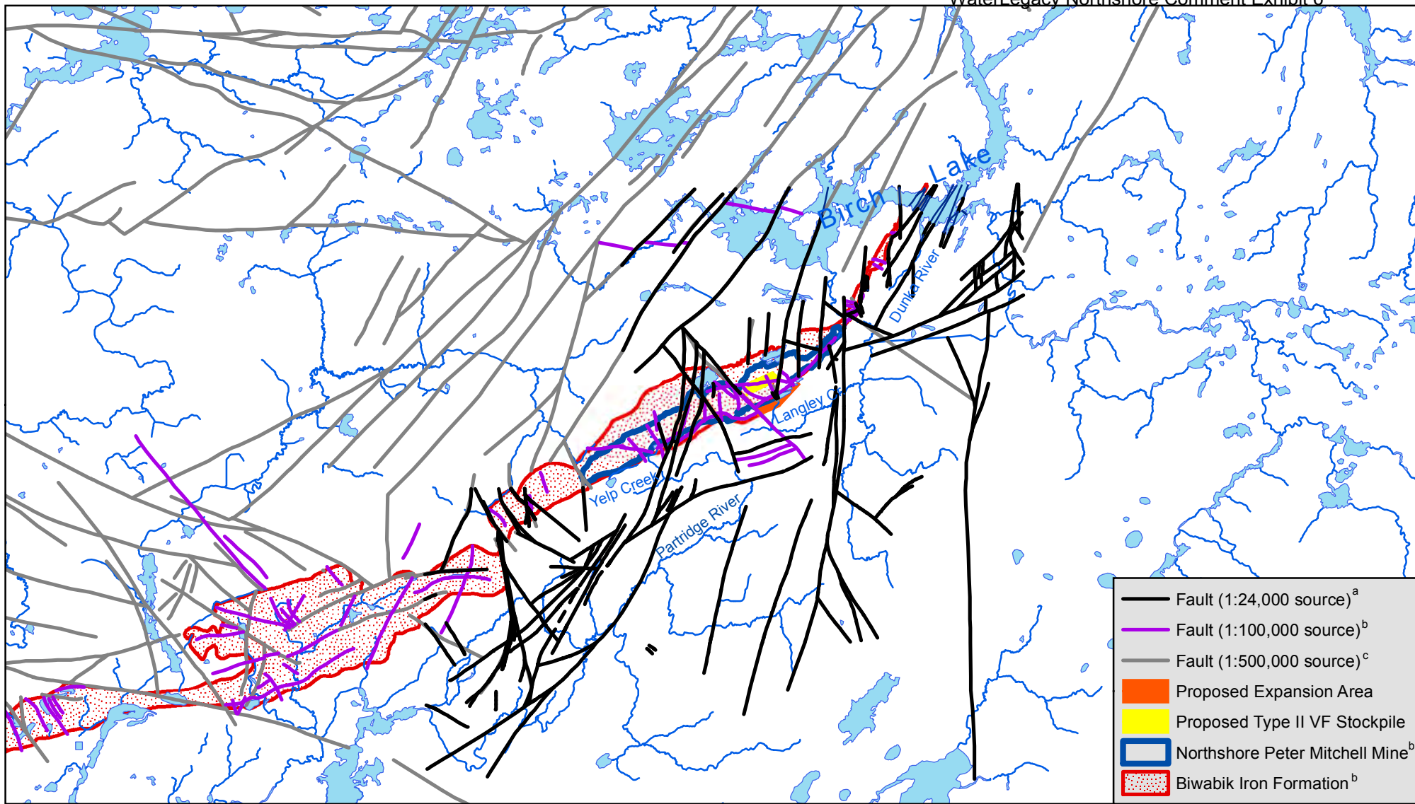
FIGURE 3 FAULTED BEDROCK AND SURFACE TOPOGRAPHY VICINITY OF PROPOSED NORTHSHORE MINING EXPANSION ST. LOUIS COUNTY, MINNESOTA
