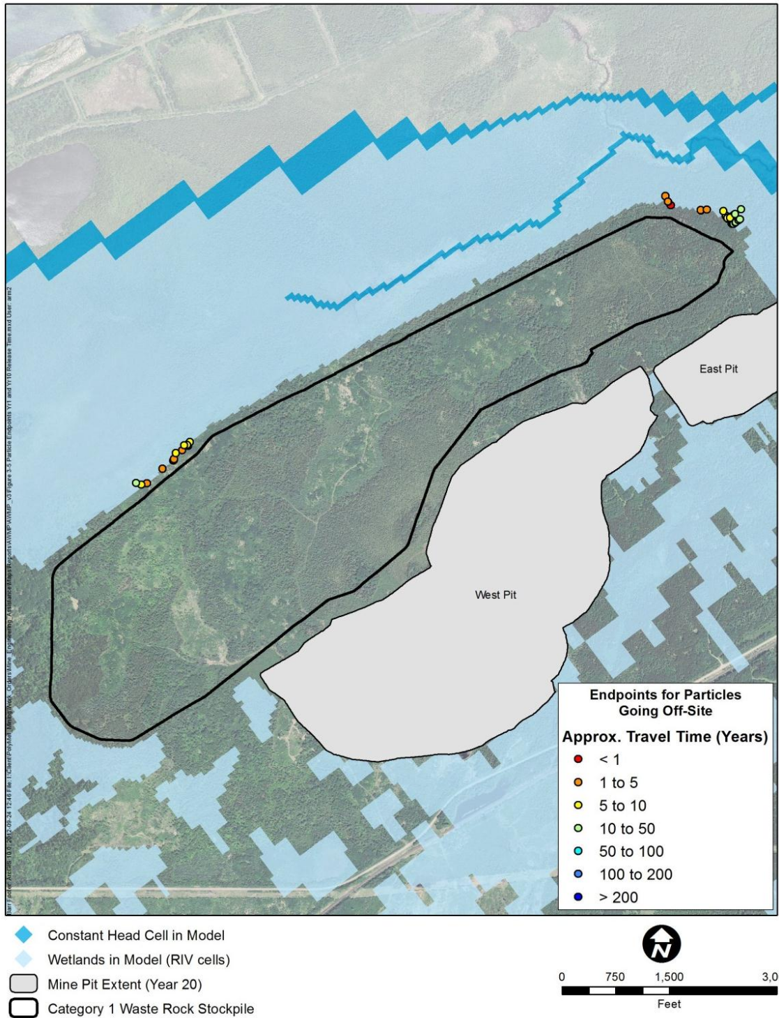
Figure 2-3 Groundwater Model (MODFLOW) Tracking of Short and Shallow Groundwater Flow Paths from Category 1 Waste Rock Stockpile Drainage
